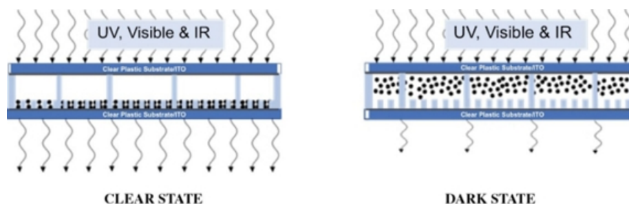
Figure 1. Schematic cross-section of electrokinetic film in clear and dark states.
